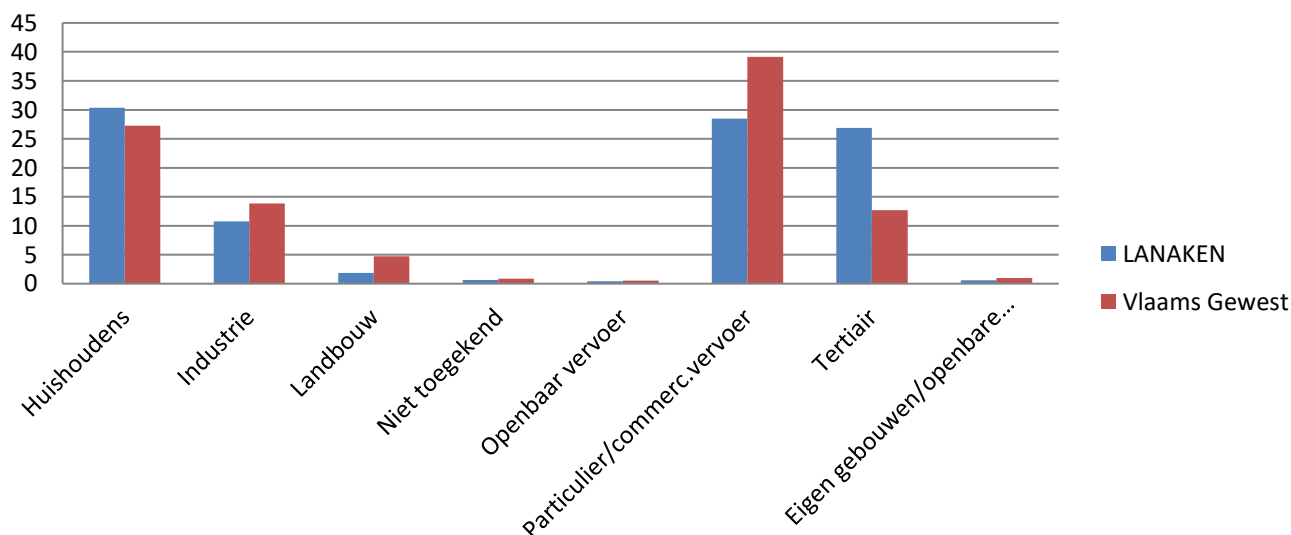
CO 2 -emissies per sector, 2022, in procenten
